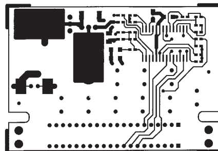
Figure 12. COMP Side
