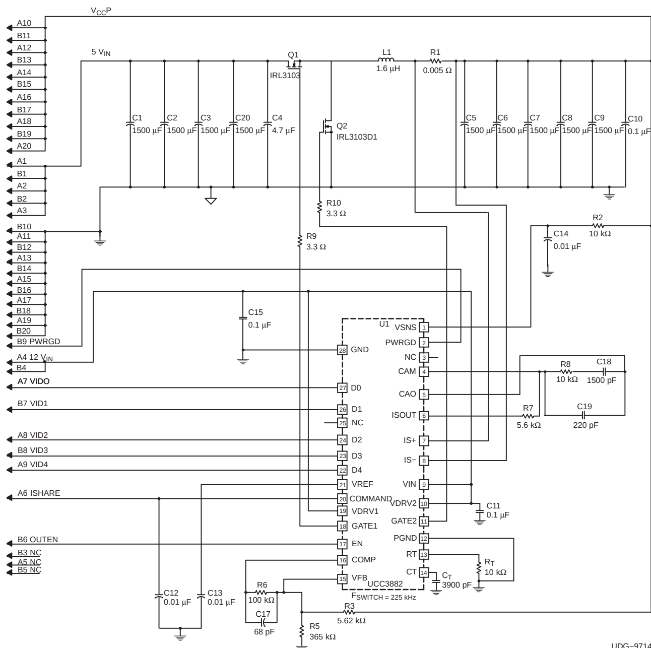
Figure 9. Reference Design – UCC3882 5-Bit Synchronous Rectifier PWM Controller for the Intel Pentium® Processor
